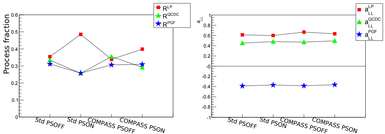
Figure 8.12: The dependence of fractions R^i (left plot) and \langle a_{LL} \rangle 's (right plot) for LO, QCDC and PGF processes on the MC settings.
