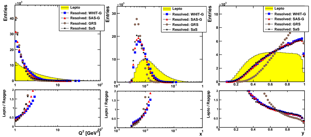
Figure 10.15: Comparison of kinematic distributions of events generated by the LEPTO with distributions of events originating from resolved photon processes obtained from the RAPGAP. Different points correspond to several selections of the photon PDFs.
