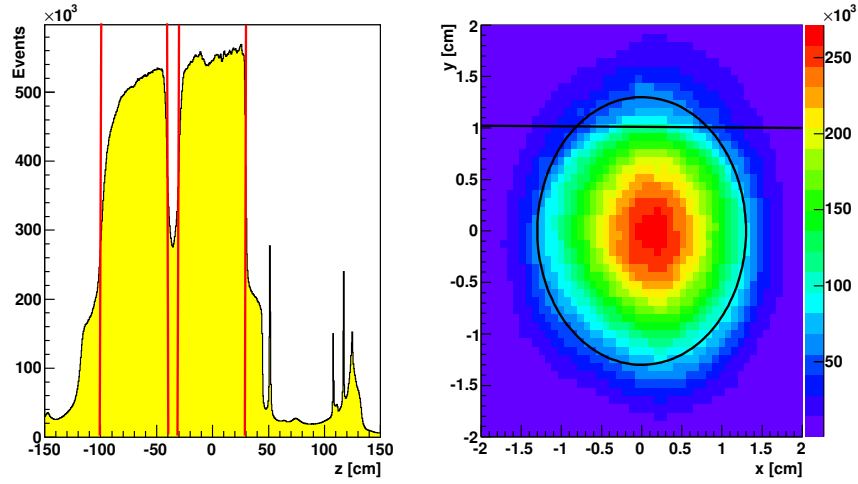
Figure 7.6: The longitudinal vertex distribution (left) with the cuts along Z coordinate ( -100 \text{ cm} < Z < -40 \text{ cm} and -30 \text{ cm} < Z < 30 \text{ cm} ) and the transverse vertex distribution (right) with cuts on Y > 1 \text{ cm} and R < 1.3 \text{ cm} .
