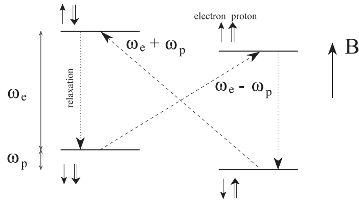
Figure 4.4: Energy levels for an e-p state in a strong magnetic field B . Arrows indicate direction of the proton \uparrow and electron \uparrow spins; \omega_p and \omega_e are Lamor frequencies of the proton and electron, respectively. Figure comes from Ref. [78].
