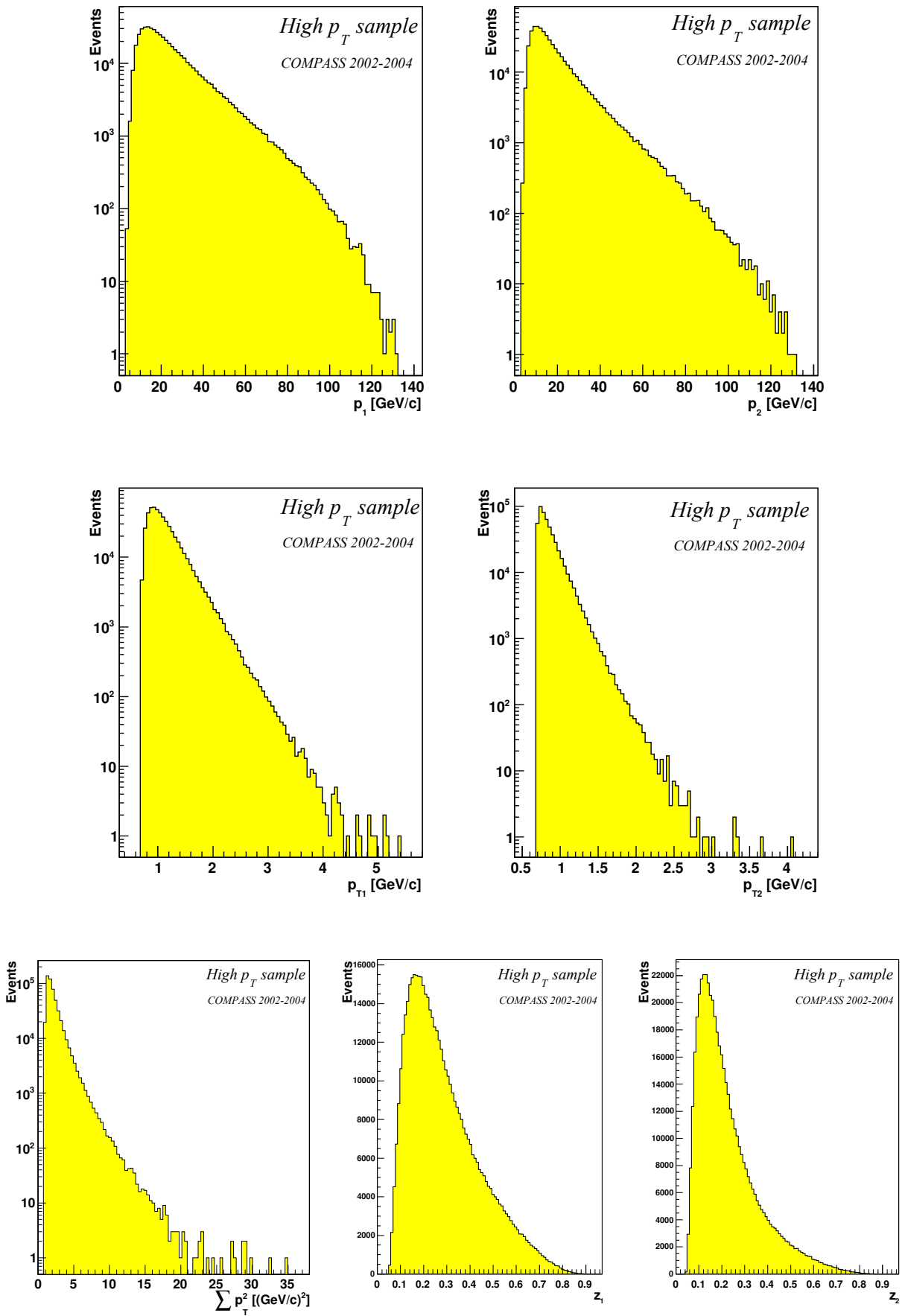
Figure 7.8: The distributions of hadron variables p_1 , p_2 , p_{T1} , p_{T2} , \sum p_T^2 , z_1 , z_2 for the high p_T data sample.
